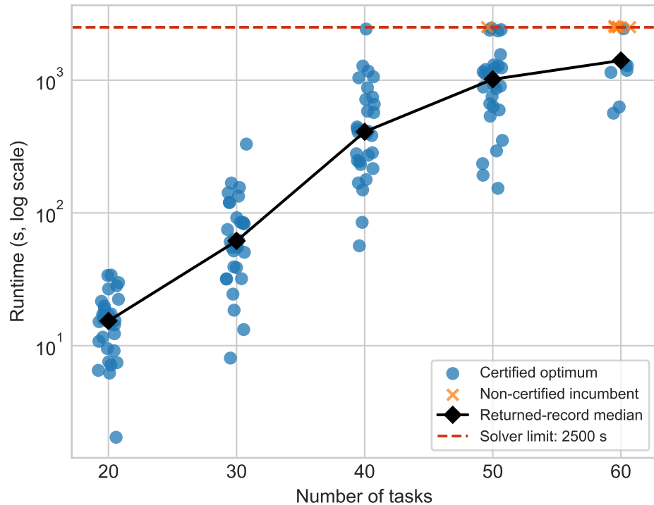
(b) Exact computational effort
